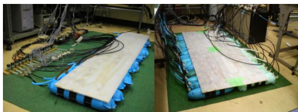
Fig.9 Photographs of pedal locomotory air matt.
